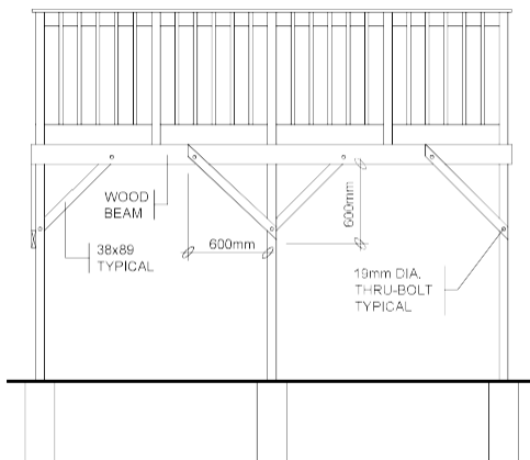
BRACING PARALLEL TO BEAM
