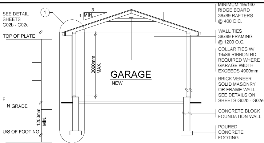
GABLE ROOF
